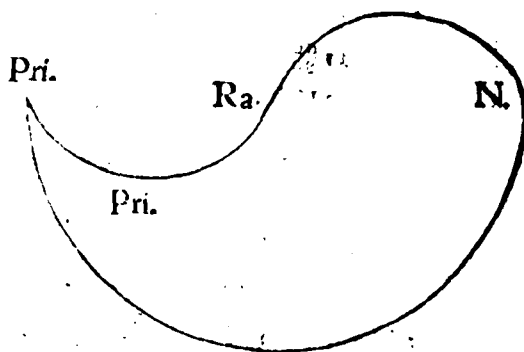
FIGVRA AEQVATIONVM.
